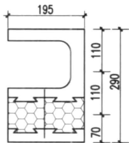
FQ-1-2 洞口块
