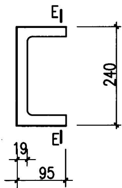
Q240-4 压顶块
